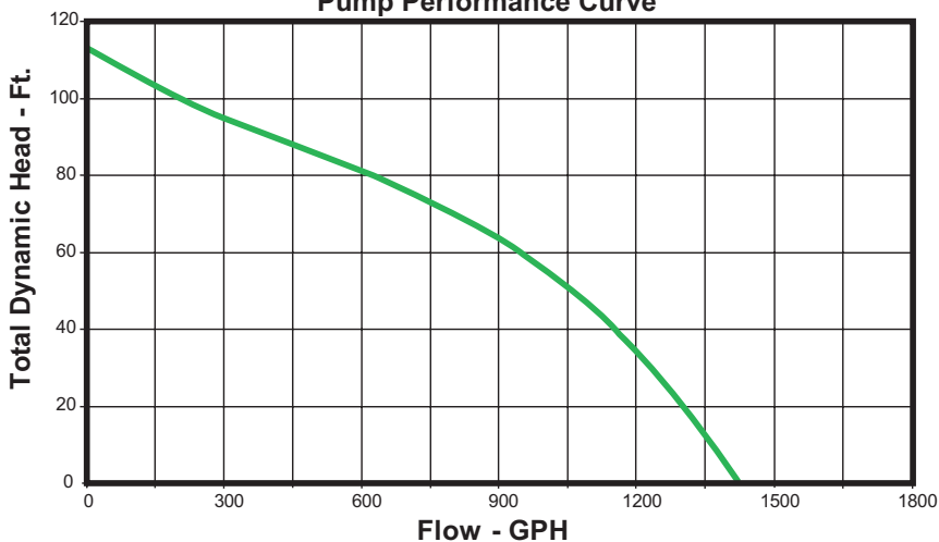
"High Capacity" Water Mover Pump Performance Curve
